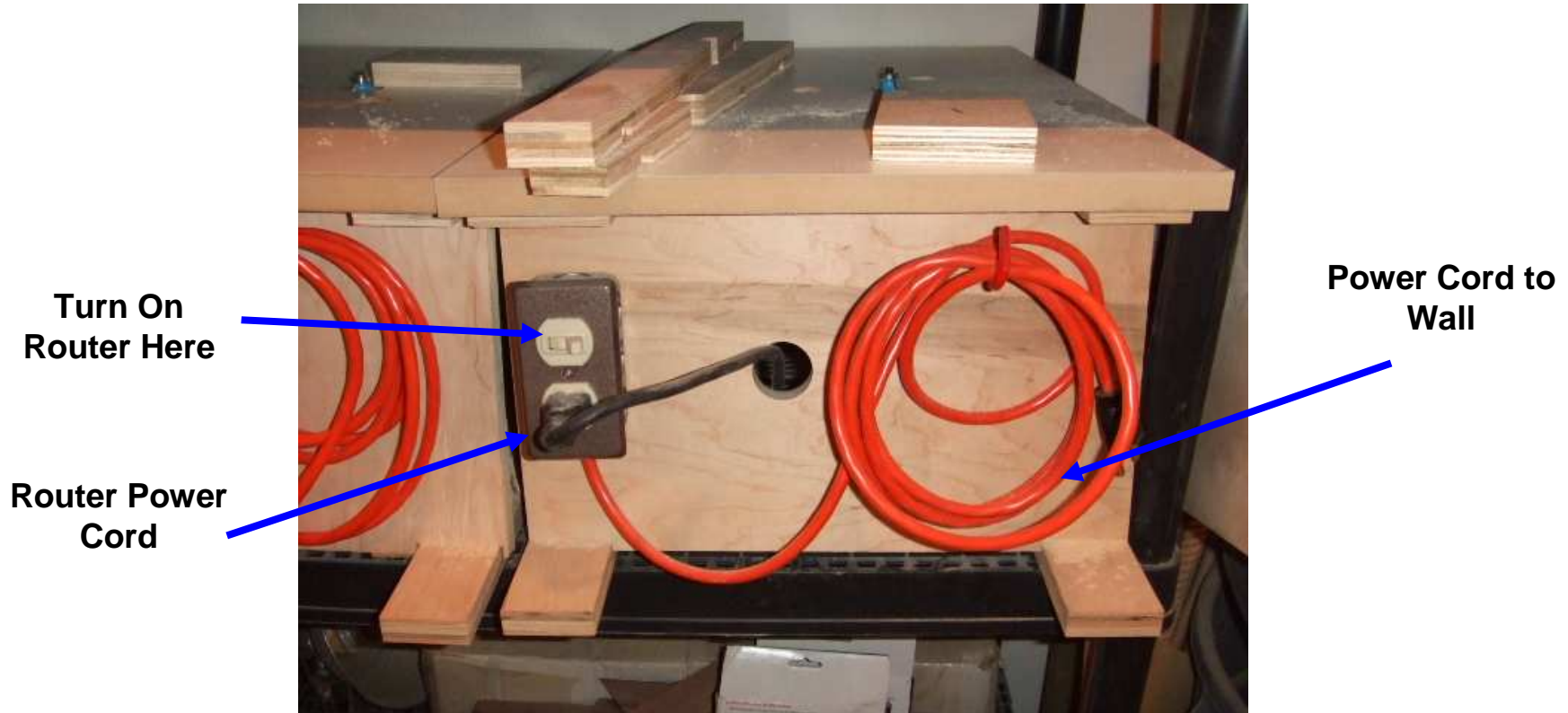
Portable Router Table Electrical Connections
