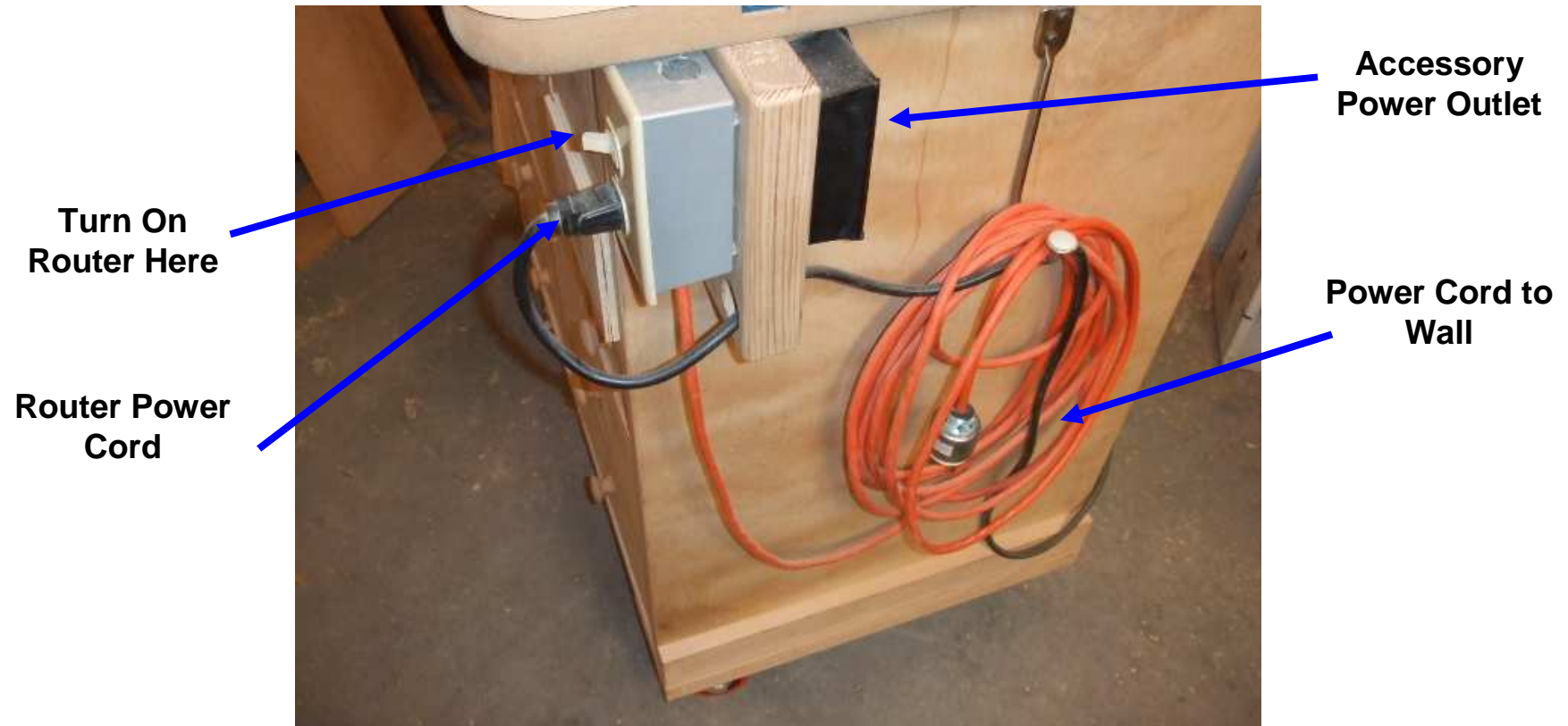
Stationary Router Table Electrical Connections
